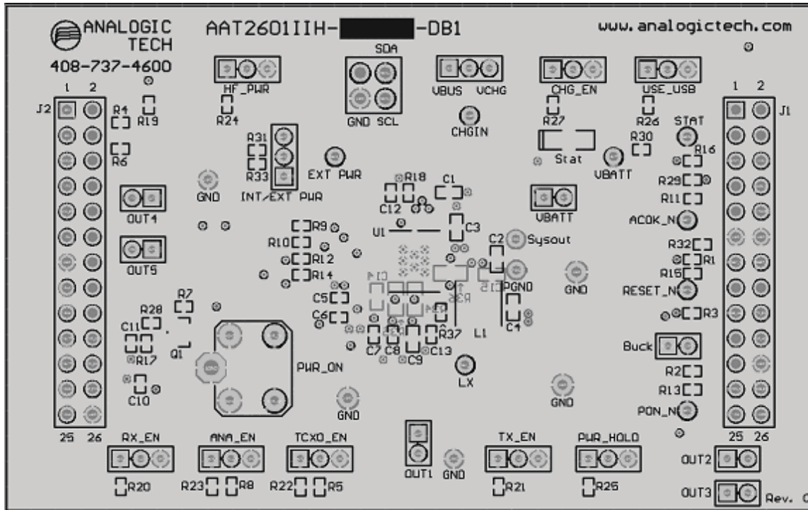
Figure 13: AAT2601B Evaluation Kit Mid2 Layer.
